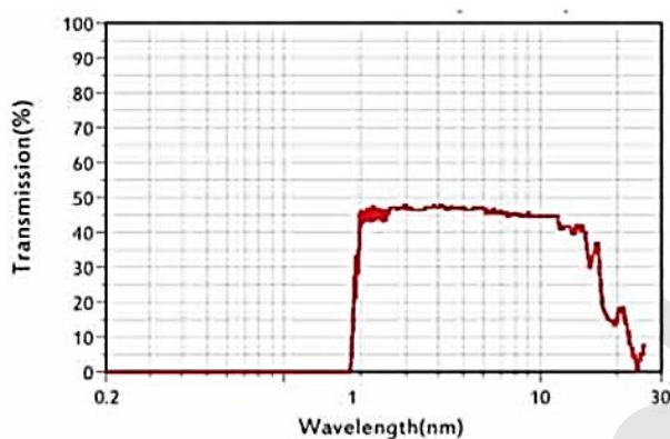
Ge Transmission
