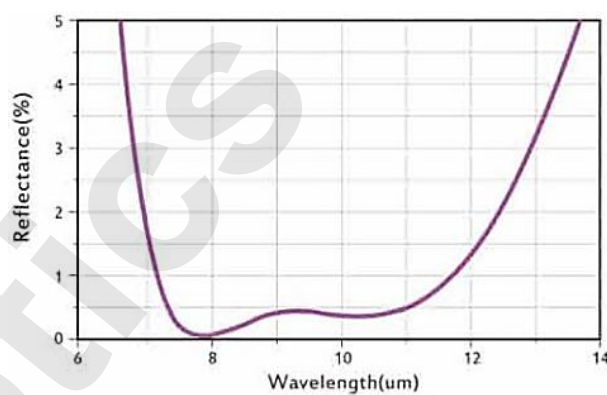
IR2 Coating @ 8~12um
